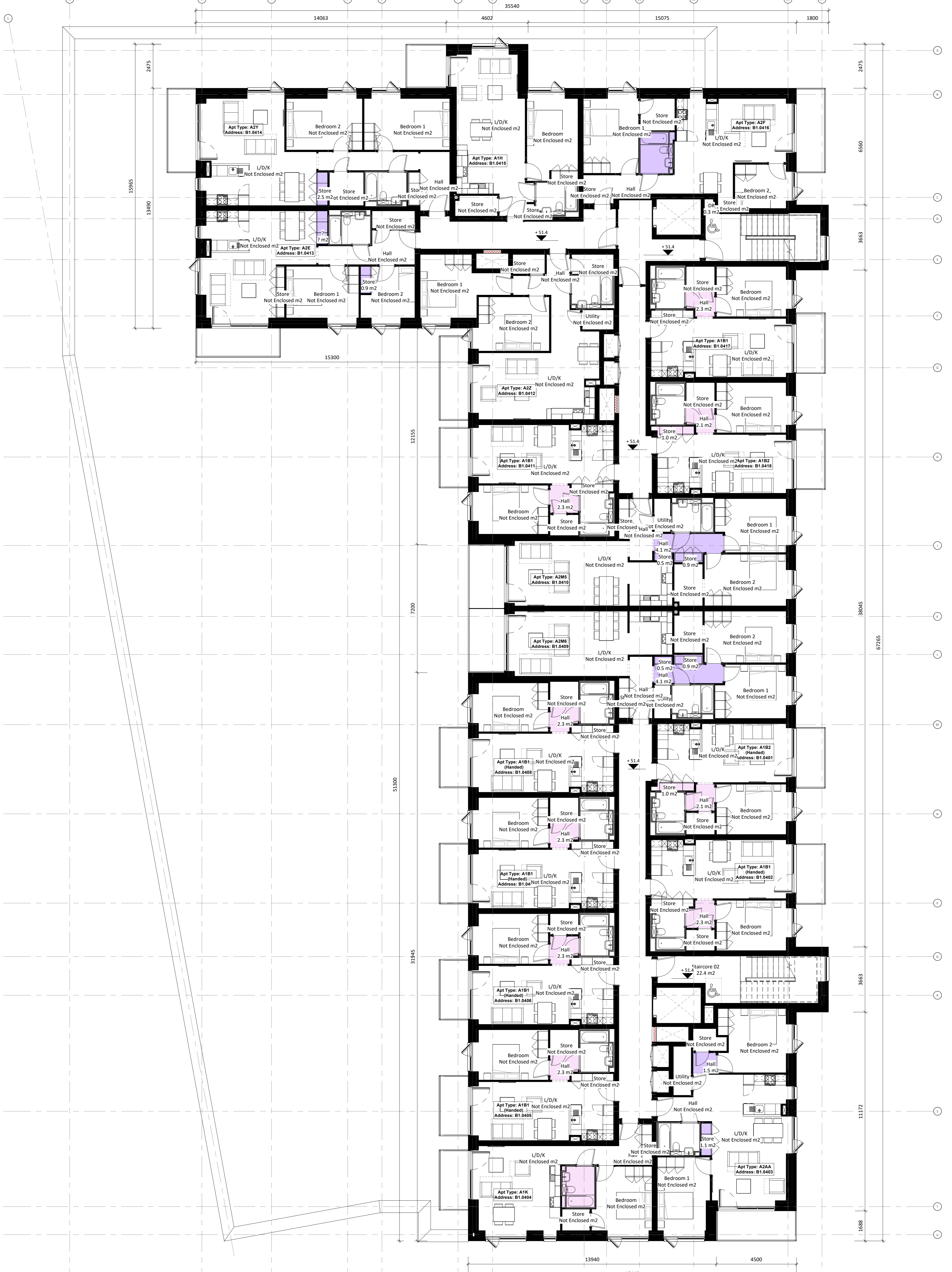
Block 01 - Fourth Floor Plan - Proposed
