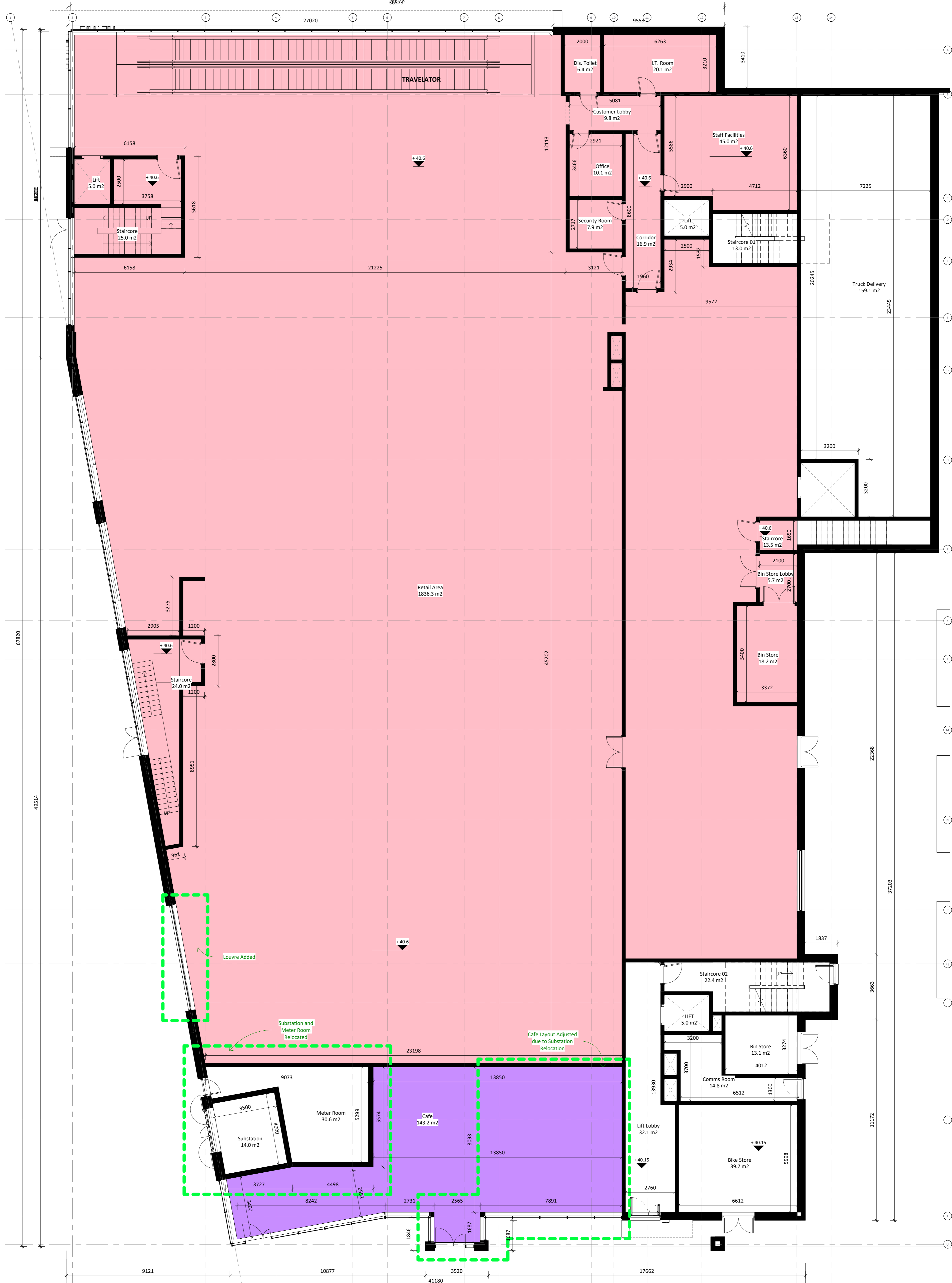
Block 01 - First Floor Plan - Proposed
